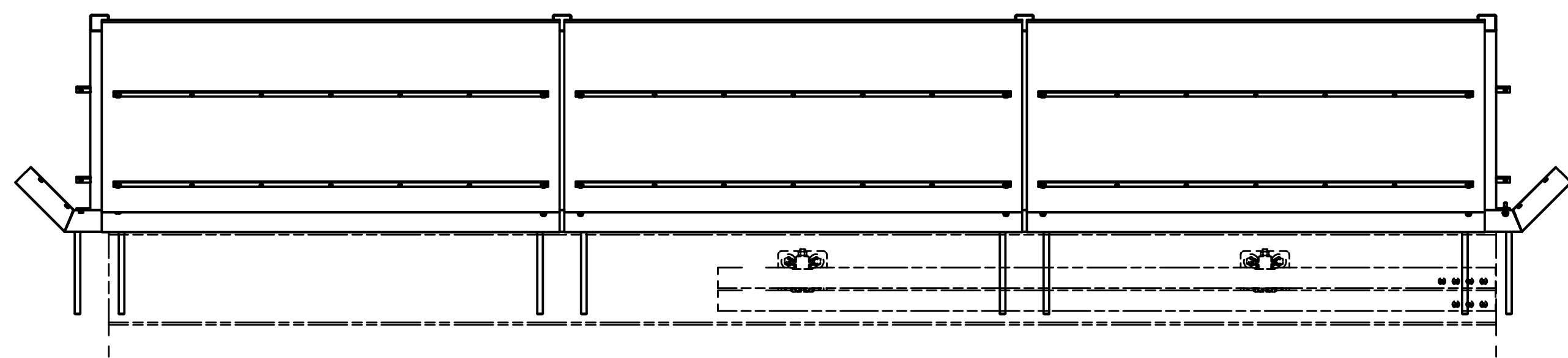
VIEW FROM TOP SCALE 1:20
