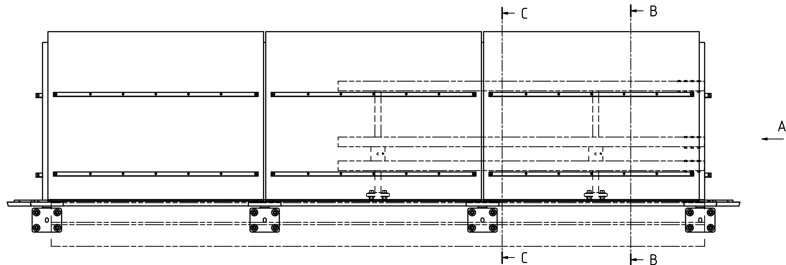
VIEW FROM INSIDE ROAD SCALE 1:20
